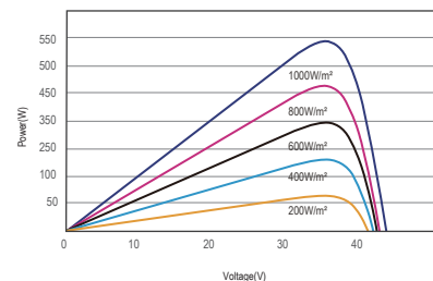
P-V Curves(540W)
