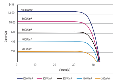
I-V Curves(540W)
